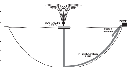
Narrow Umbrella Nozzle
